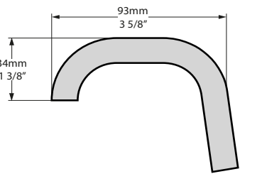
Rim Detail
