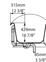
Section BB
